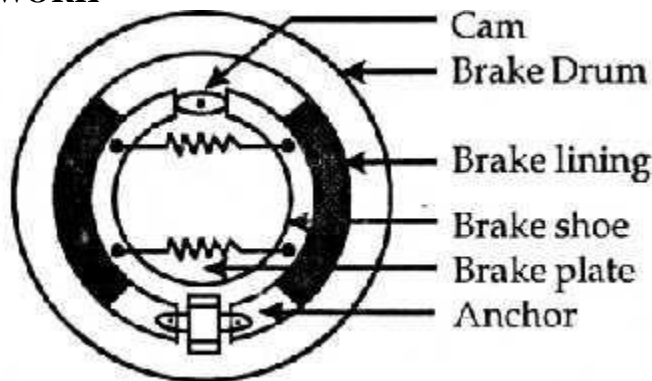
Mechanical drum Brake
