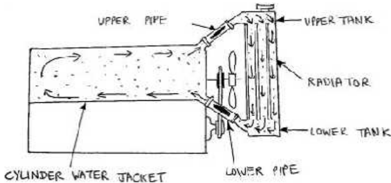
Thermosiphon water cooled system
