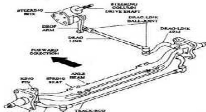
Front Axle
