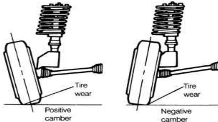
Camber angle
