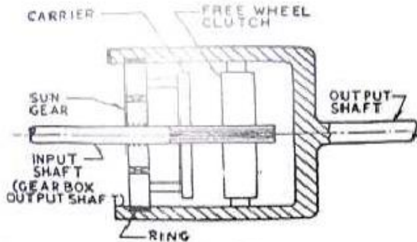
Overdrive
