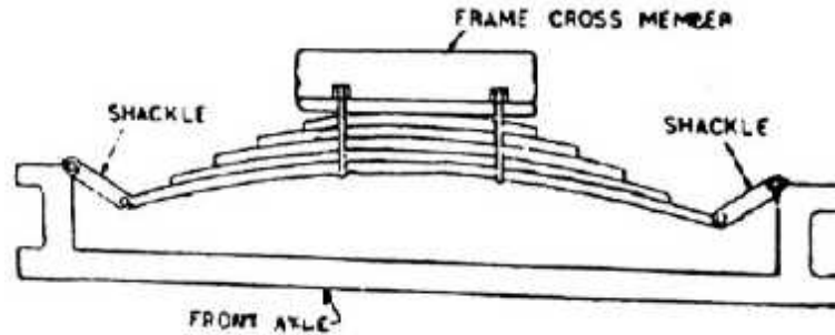
Transverse Spring
