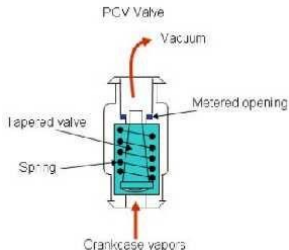
Positive Crankcase Ventilation
