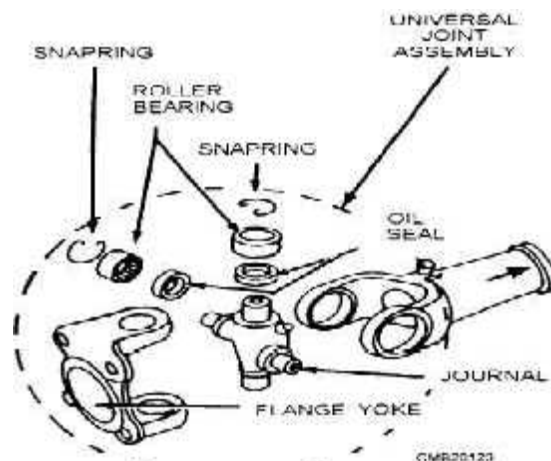
Cross and roller universal joint - disassembled view.
