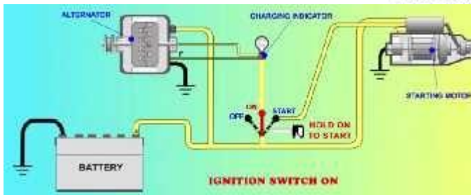
Alternator Case
