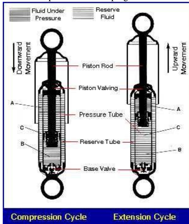
Shock absorber
