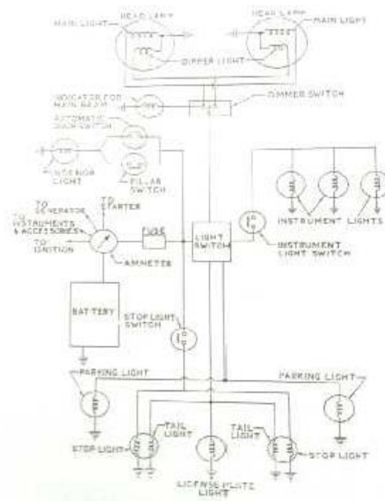
Lighting circuit
