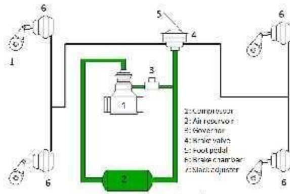
Basic Air Brake System
