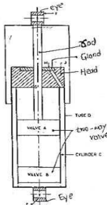
Telescopic absorber
