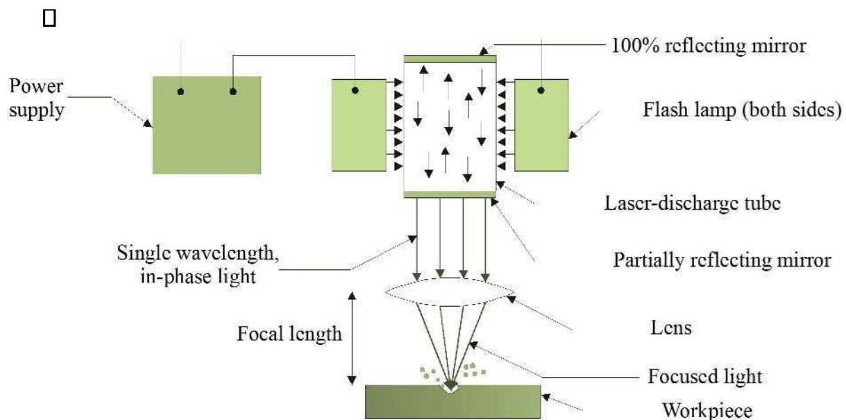
Figure 17: Laser beam machining schematic
